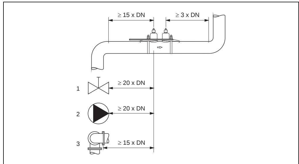
Inlet and outlet runs (top view)
